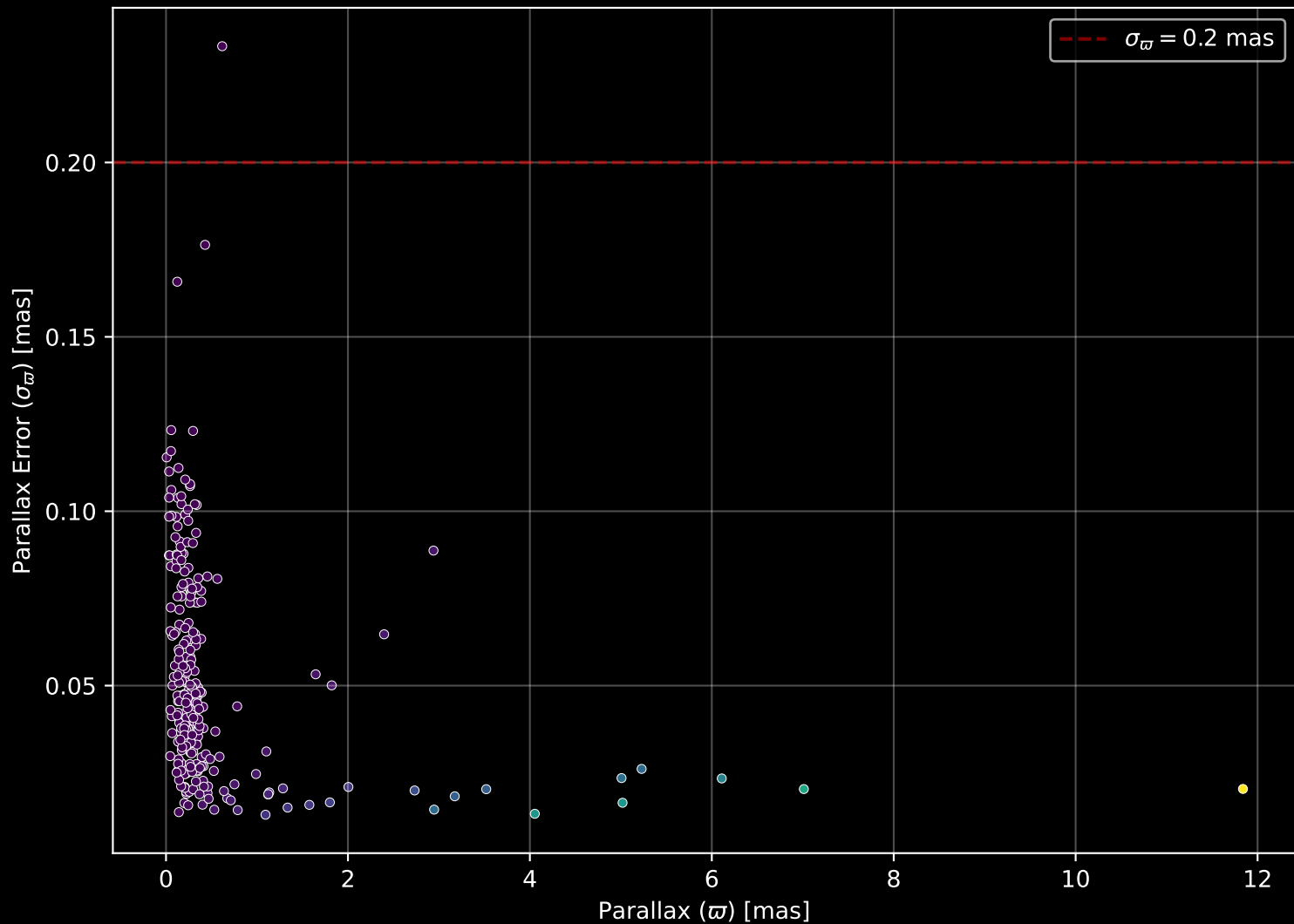
APOGEE DR17 Field: [146+00] Parallax Quality (n= 268)
