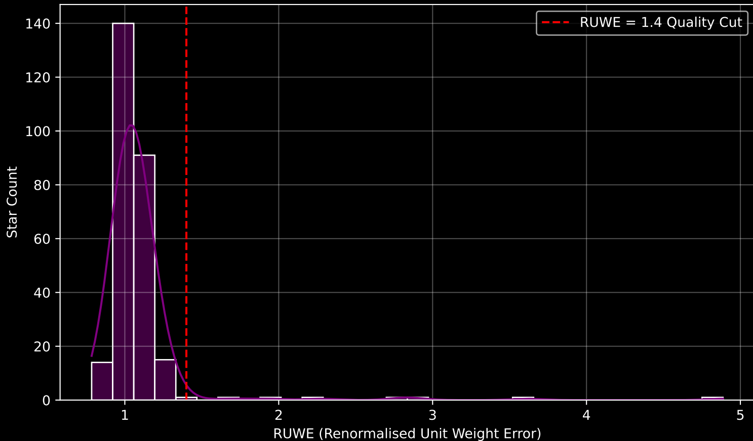
GAPOGEE DR17 Field [146+00] RUWE Distribution (n= 268)
