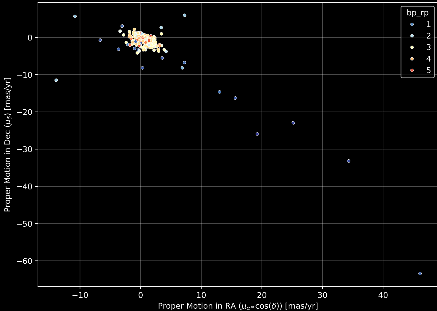
APOGEE DR17 Field: [146+00] Proper Motion Diagram (n= 268)
