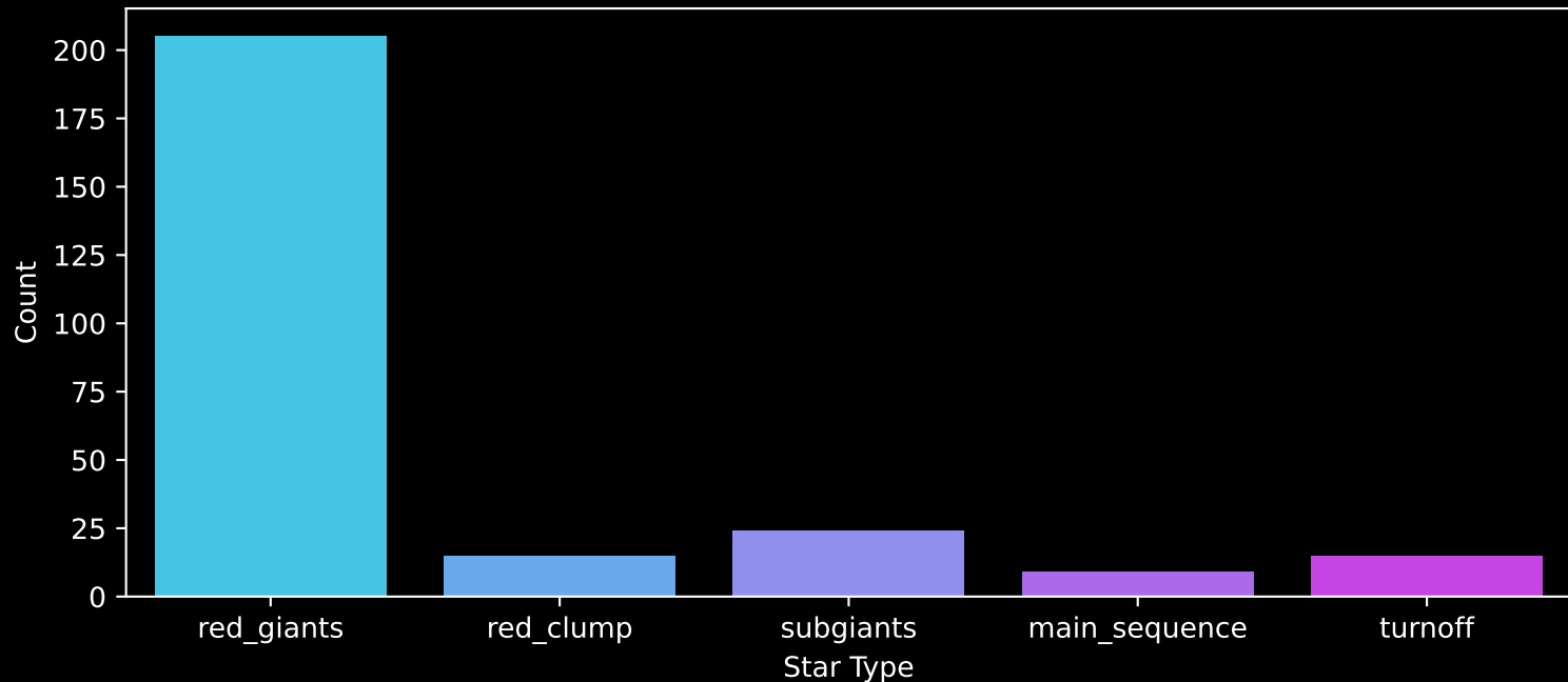
APOGEE DR17 Field: [146+00] Count plot of Star Type
