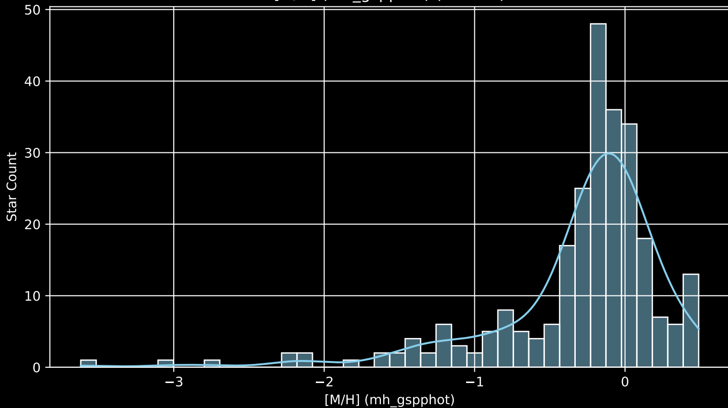
APOGEE DR17 Field: [146+00 [M/H] (mh_gspphot) (n= 261)
